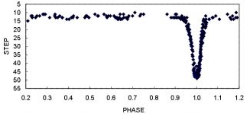
Figure 1. The phased visual light curve of LD 282, based on 341 observations by Guilbault.
