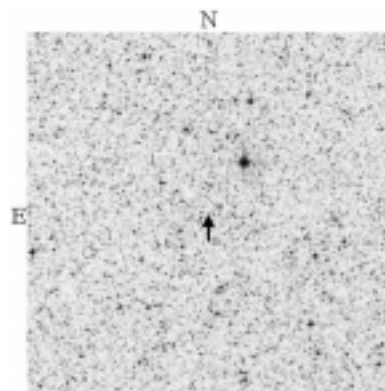
Figure 9. HU Sgr.
