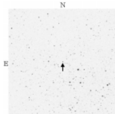
Figure 4. VW Sgr.
