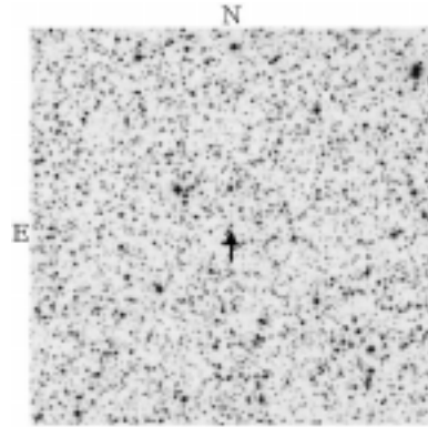
Figure 1. NY Cyg.
