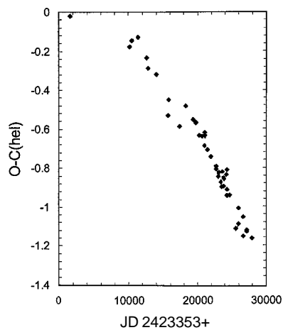
Figure 3. QX Cyg: O-C Graph.
