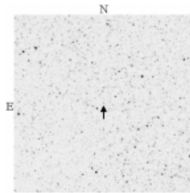
Figure 6. GZ Sgr.
