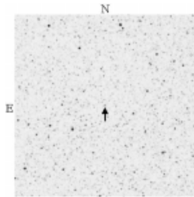
Figure 5. GW Sgr.
