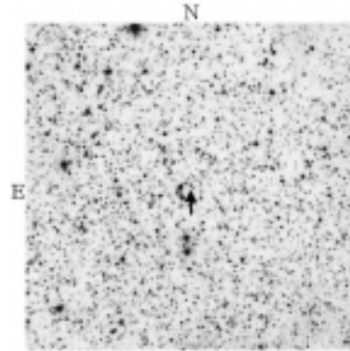
Figure 2. QX Cyg.
