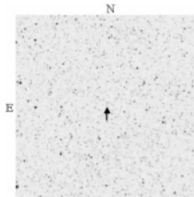
Figure 7. HK Sgr.
