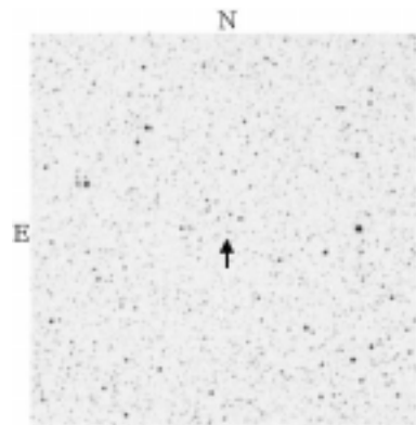
Figure 8. HT Sgr.
