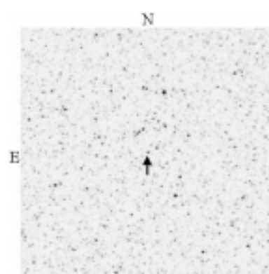
Figure 10. HW Sgr (see text for discussion on identification of the variable).
