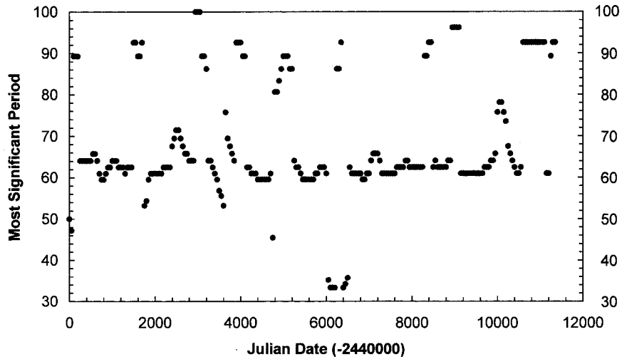
Figure 2. The most significant period of EU Del, as a function of time, based on wavelet analysis of 5-day means of AAVSO visual data. The 62.5-day known period is usually dominant. The 95 \pm 5 -day period is probably an artifact of irregularity, systematic error, and sparse data during seasonal gaps, as explained in the text.
