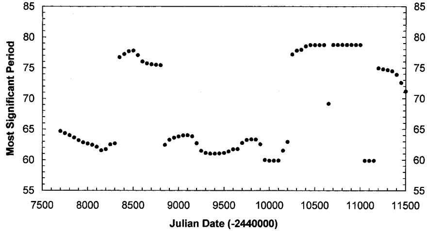
Figure 1. The most significant period of EU Del, as a function of time, based on wavelet analysis of AAVSO Photoelectric Photometry data. The 62.5-day known period is usually dominant. The 77 \pm 2 -day period is probably an artifact of irregularity and seasonal gaps, as explained in the text.
