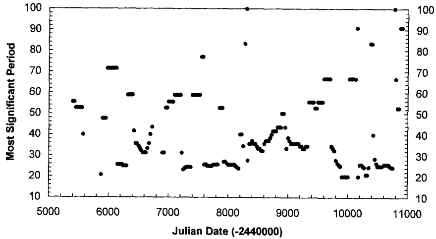
Figure 3. The most significant period of W Boo, as a function of time, based on wavelet analysis of AAVSO Photoelectric Photometry data. A histogram of these results shows peaks at 25, 35\pm 3 , and 55\pm 3 days—all of these consistent with previous results using Fourier analysis (Percy and Desjardins 1996).
