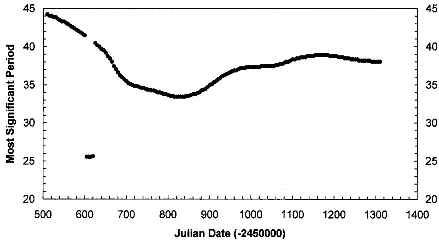
Figure 4. The most significant period of SX UMi, as a function of time, based on wavelet analysis of CCD photometry provided by Josep M. Gomez Forrellad and Enrique Garcia Melendo. A period of about 38 days is present; this value is consistent with the results of autocorrelation analysis. The apparent “wandering” of the period, with time, is probably due to multiperiodicity or irregularity, as explained in the text.
