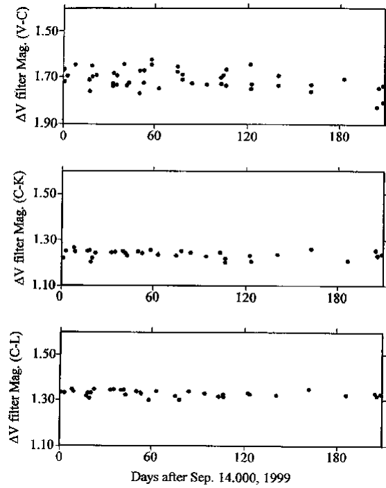
Figure 2. Plots of the V-C, C-K, and C-L magnitudes versus days after Sep. 14,000, 1999 (JD 2451436); V, C, K, and L refer to the magnitudes of RX Cep, comparison star (HD 4853), check star K (HD 5848), and check star L (HD 166205), respectively.
