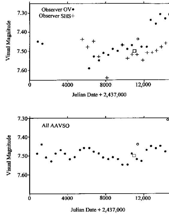
Figure 3. Plots of 500-day averages of visual magnitude versus Julian date for AAVSO observers OV and SHS (top), and all AAVSO data (bottom). Photoelectric V measurements by Zsoldos and Schude are plotted as open circles. Hipparcos values are plotted as an open square.
