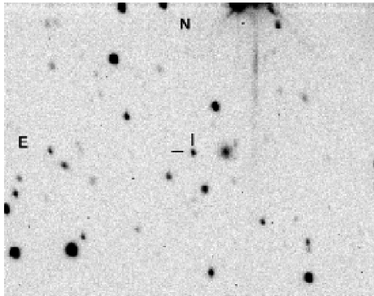
Figure 3. The field of GRB030323. Image taken with the NOFS 1.0m telescope on 030324 with an Rc filter. Field of view is 3 \times 4 arcmin, with the afterglow marked.
