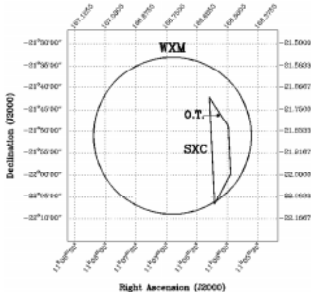
Figure 2. The sky map showing the location of the HETE WXM and SXC error boxes, along with the location of the optical transient. Taken from Graziani et al. (2003).
