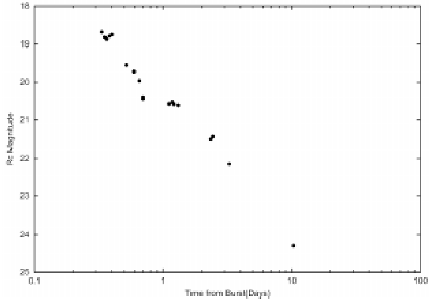
Figure 4. The R_c light curve for GRB030323. Additional early-time unfiltered data are included after adjustment onto the R_c system.
