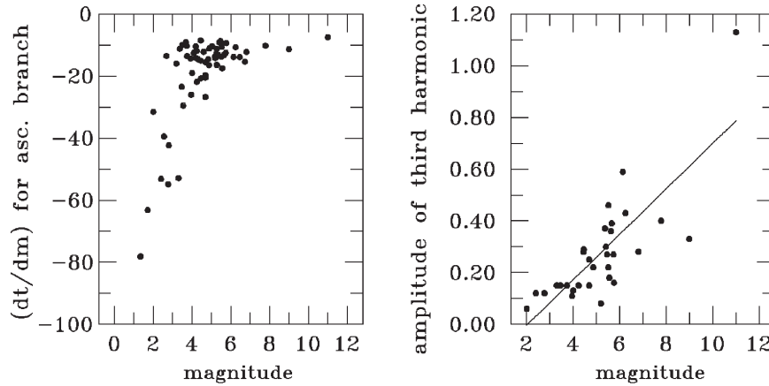
Figure 1. Left : the diagram dt / dm (for the ascending branch) vs. \Delta m . Right : the diagram r_3 vs. \Delta m .
