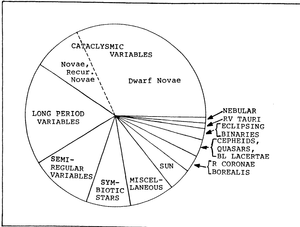
Figure 2. Types of variable stars for which data were requested during the fiscal year 1982-83.
